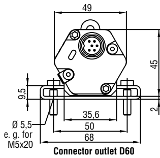
Connector outlet D60
