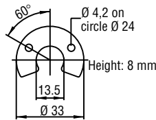
Composite PA-Ferrite-GF20 Weigth ca. 11g Operating temperature: -40 ... +100°C
