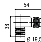
6 pin 90° female connector M16 insert adjustable in 45° positions Part No. ST C0 9131-6
